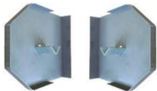
15"x15" Hex End Bracket with Welded Spring Support 3/32" or 1/8" thickness
